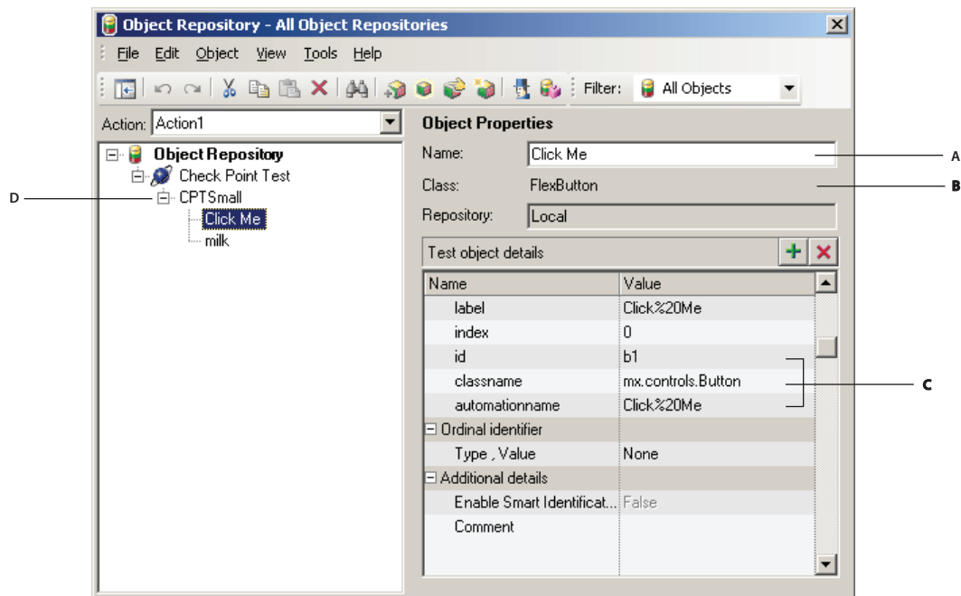
A. Test object name B. Test object model class C. Flex properties used to identify this object D. Application hierarchy
